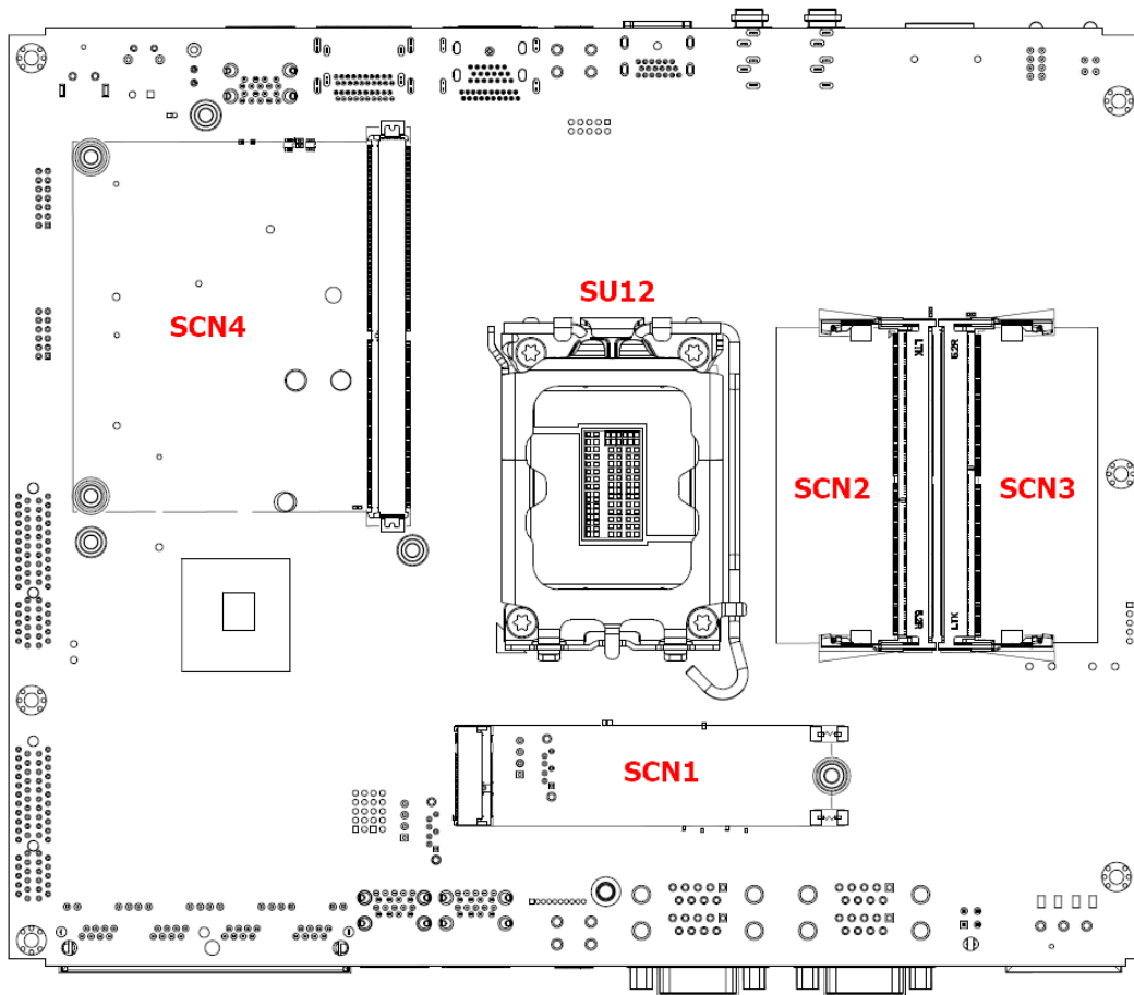
PSB516 Top View
