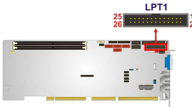
Figure 3-16: Parallel Port Connector Location
